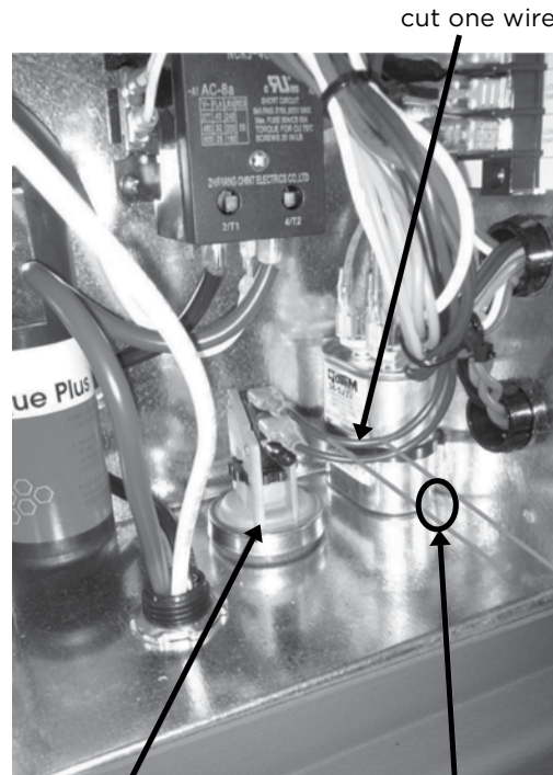
Pressure Switch
